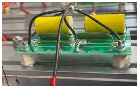
PCB-Stützisolator
